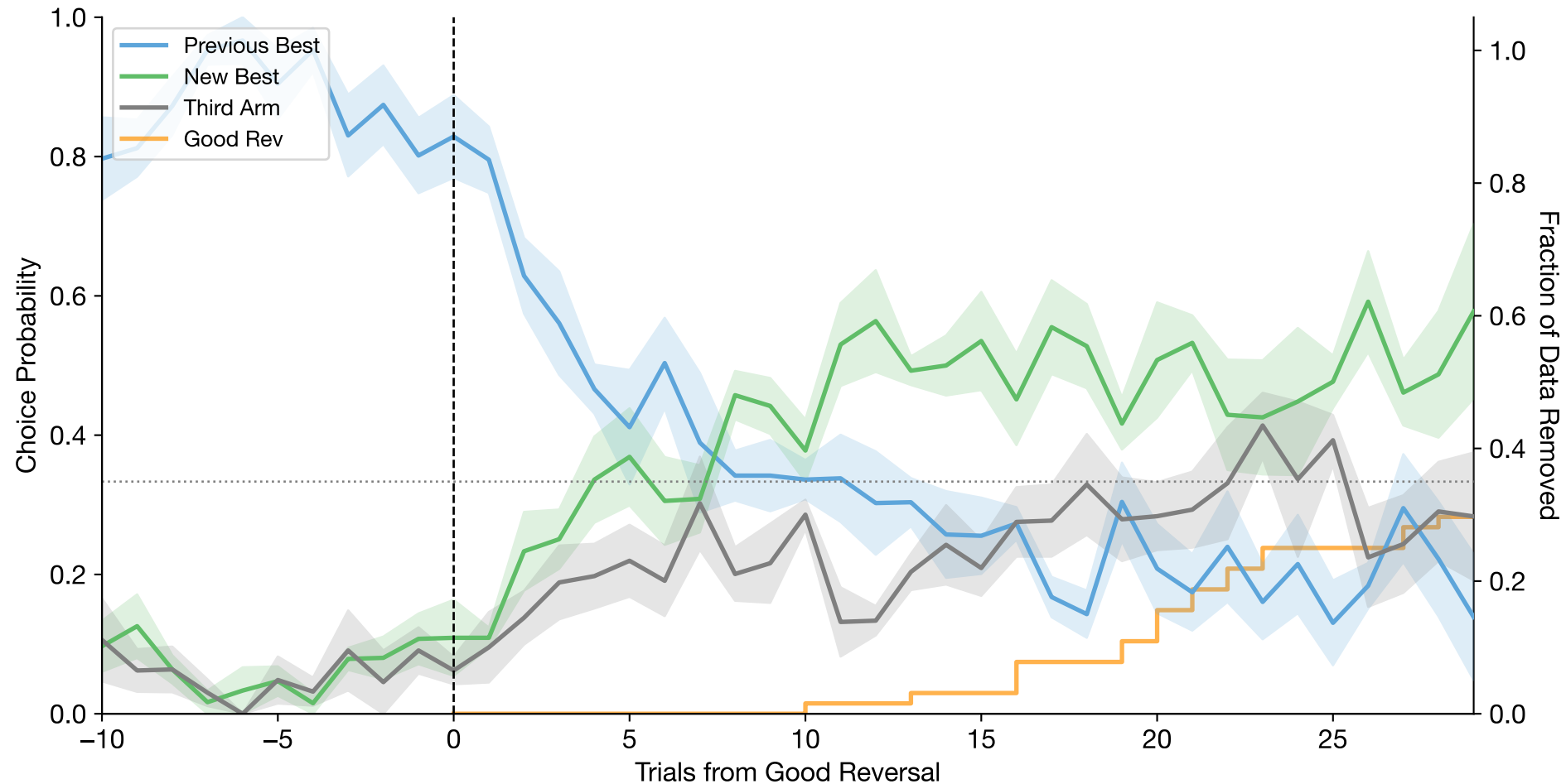
Good Reversal-Aligned Choices (mean \pm se across subjects | n=6 subjects, n=64 reversals)
